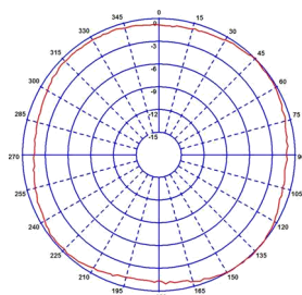
Typical Polar Plot (Picture 360MHz)
