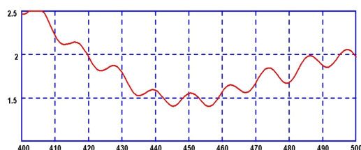
Typical VSWR v Frequency (Picture 460MHz)
