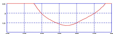
Typical VSWR v Frequency (Picture 455MHz)
