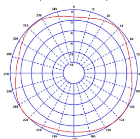
Typical Polar Plot (Picture 460MHz)
