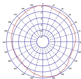
Typical Polar Plot (Picture 455MHz)
