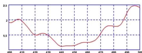
Typical VSWR v Frequency (Picture 451MHz)
