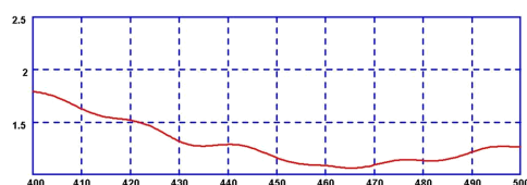
Typical VSWR v Frequency (Picture 460MHz)
