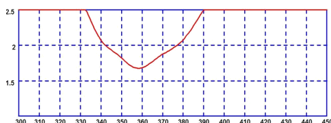
Typical VSWR v Frequency (Picture 360MHz)
