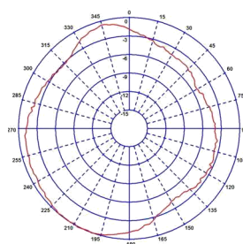
Typical Polar Plot (Picture 360MHz)
