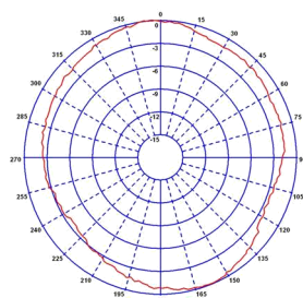
Typical Polar Plot (Picture 455MHz)
