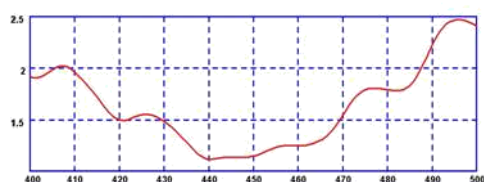
Typical VSWR v Frequency (Picture 451MHz)
